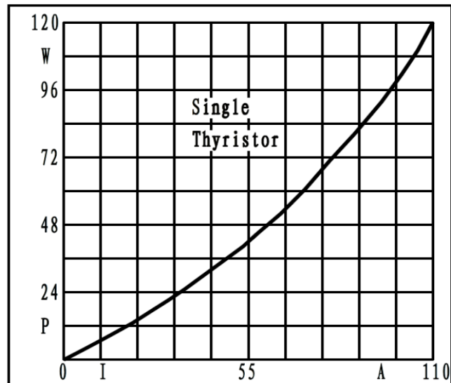
Fig3. Power dissipation
